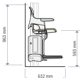
Side view - unfolded chair
