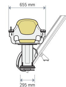
Front view - chair width
